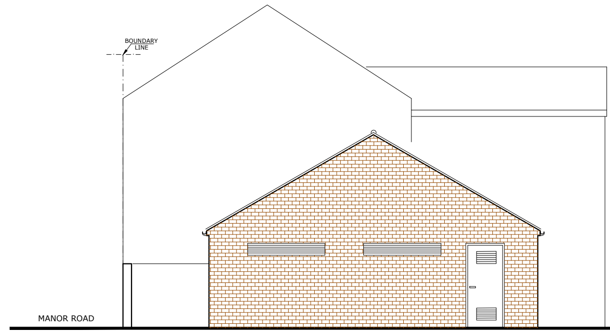
PROPOSED REFUSE STORE (SIDE ELEVATION) SCALE: 1/100 @A3
