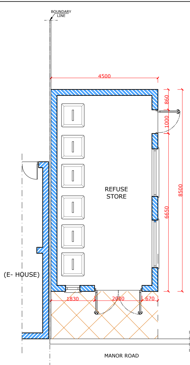
PROPOSED REFUSE STORE (GROUND FLOOR PLAN) SCALE: 1/100 @A3
