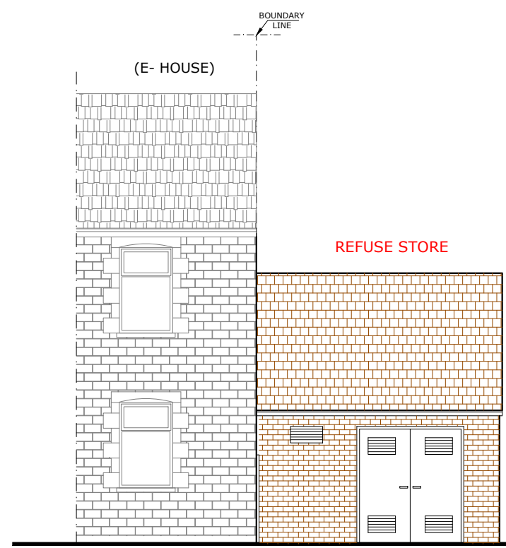
PROPOSED REFUSE STORE (FRONT ELEVATION) SCALE: 1/100 @A3
